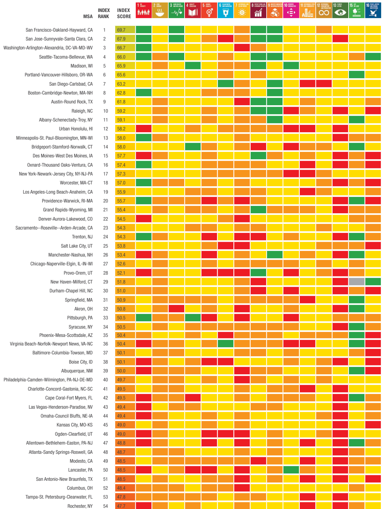
FIGURE 2: DASHBOARD
